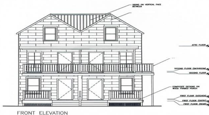
FRONT ELEVATION
