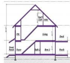
SECTION @ FOYER
